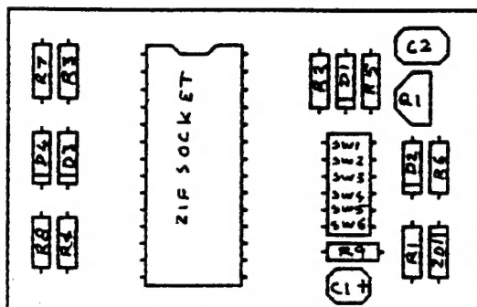
component overlay
